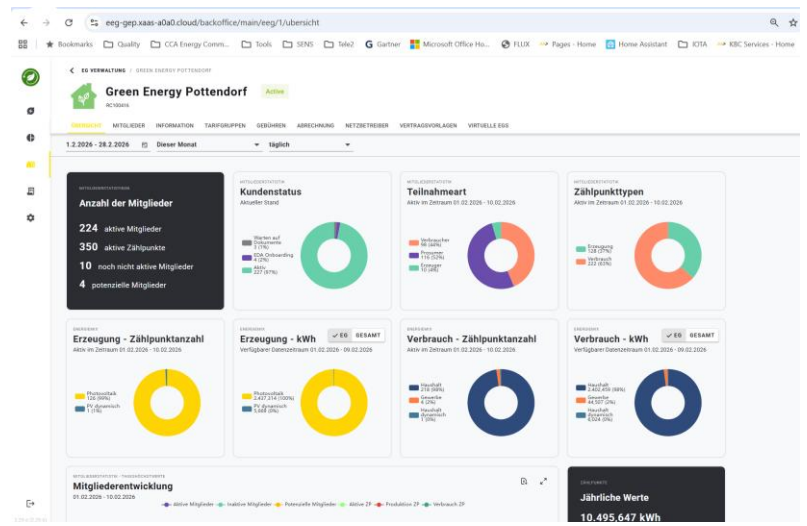
Backoffice
